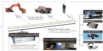
Pipeline third-party intrusion detection
